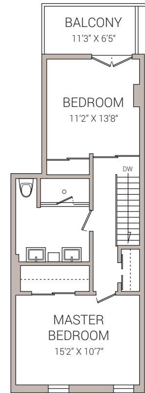
SECOND FLOOR ALT. LAYOUT
