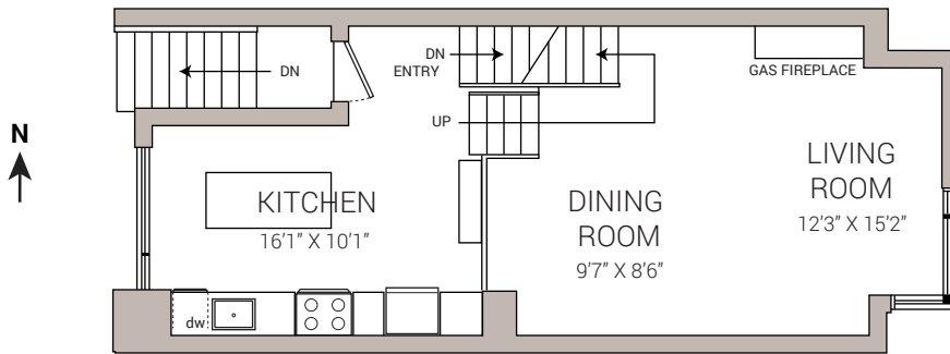
MAIN FLOOR
