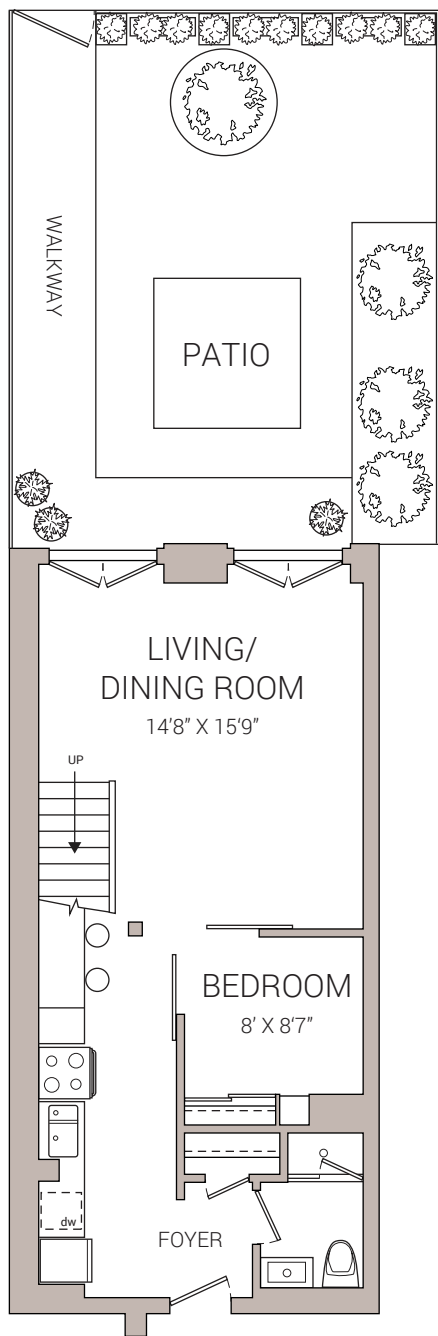
MAIN FLOOR
