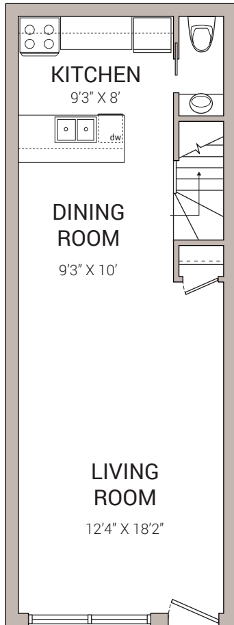
MAIN LEVEL
