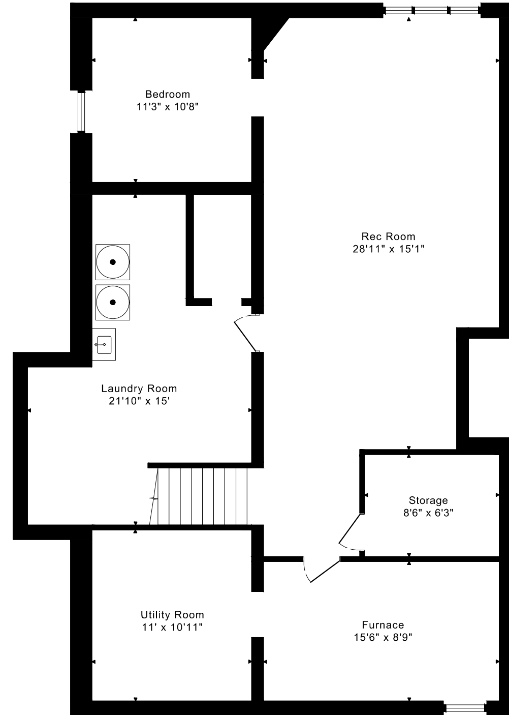
LOWER FLOOR 1450 SQUARE FEET
